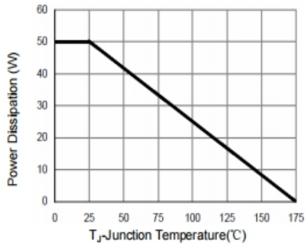
Figure 9 Power De-rating
